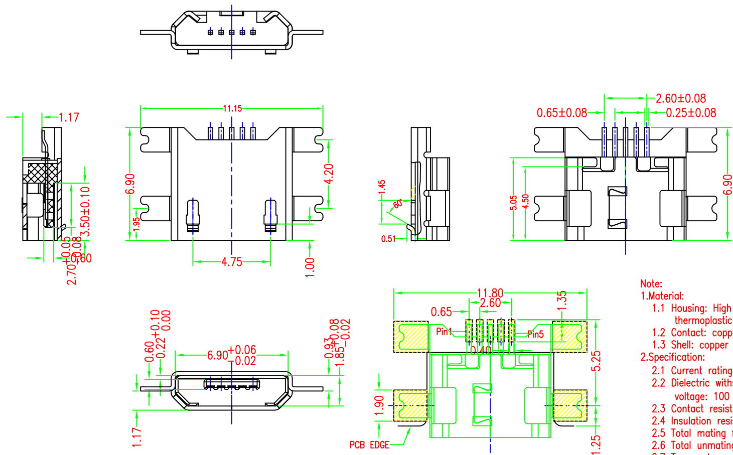
RECOMMENDED PCB LAYOUT PCB图仅供参考
